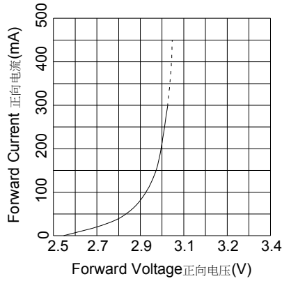
Volt-Ampere Characteristics
