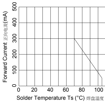
Soldering Temperature VS. Forward Current
